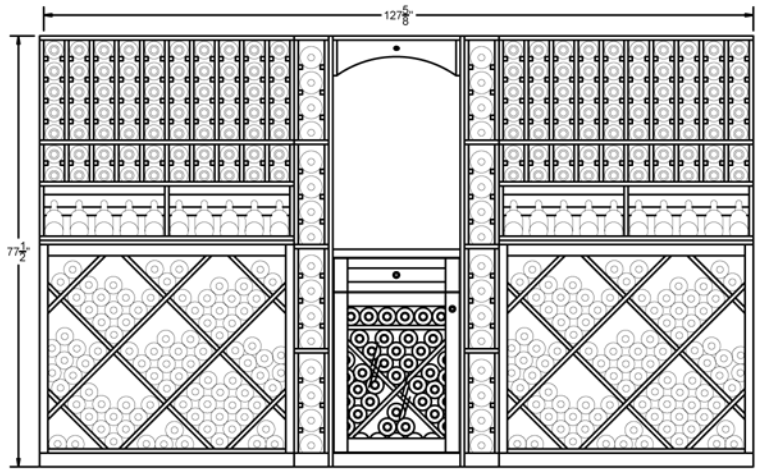
ELEVATION -A-
