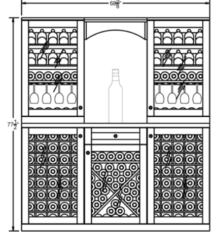
ELEVATION -B-
