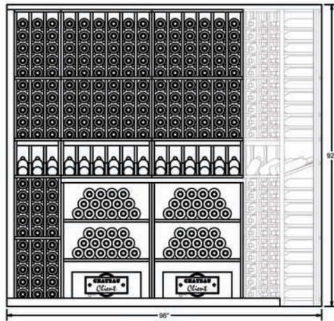
ELEVATION -A-
