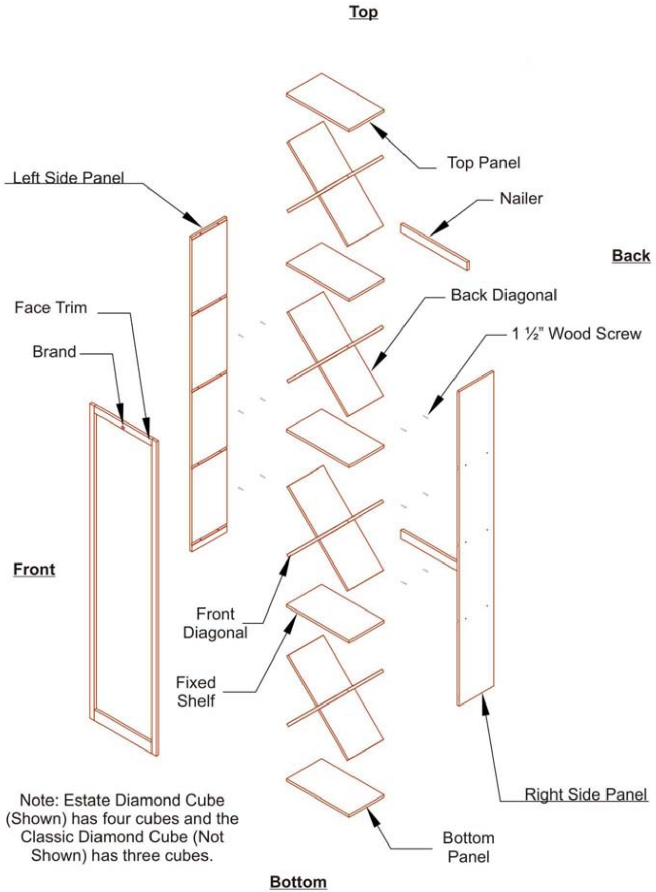
Exploded View
